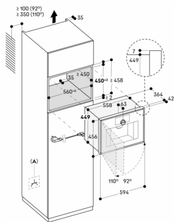
A: Accessible electrical connection Measurements in mm
