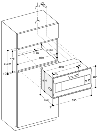
Socket measurements in mm
