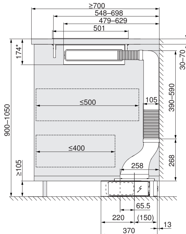
Wall/island installation with depth of \geq 700 mm
