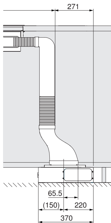
Variant with rotated fan motor
